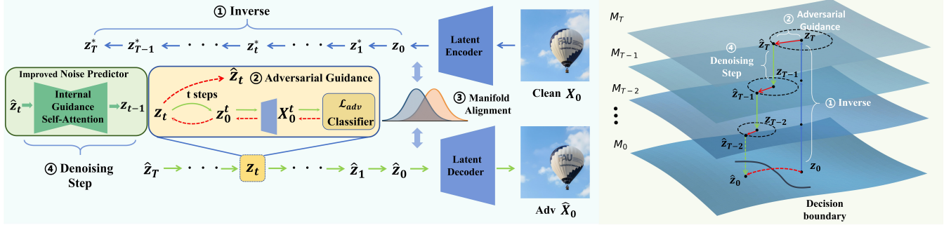
Figure 2: Overview of the proposed HAM framework. ① Inversion : A high-fidelity inverse trajectory \{z_t^*\}_{t=0}^T is first derived from the clean image using a high-order ODE solver; ② Adversarial Guidance : At each timestep t , an adversarial gradient is computed using the current latent z_t . This gradient is then projected onto the manifold to create a raw adversarial push \delta_t ; ③ Manifold Alignment : The perturbed latent \hat{z}_t = z_t + \delta_t is dynamically aligned with its clean reference z_t^* by matching their statistical properties (mean and variance), resulting in the final aligned latent \hat{z}_t ; ④ Denoising Step : A prompt-free, self-attention-guided denoising step is performed on \hat{z}_t to compute the latent for the next timestep z_{t-1} and ensure structural consistency, which repeats until the adversarial image is generated.
