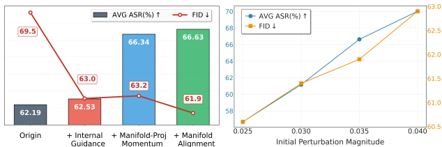
Figure 6: Ablation studies. Left: effectiveness of individual components; Right: Impact of initial perturbation magnitude. Sensitivity analysis for key hyperparams (reconstruction starting point, momentum coefficient) in Appendix D.
